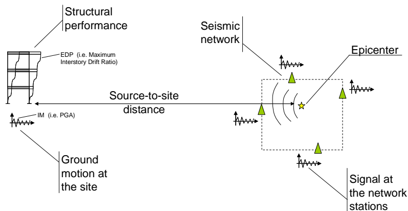
Figure 1: Regional EWWS for structure-specific applications
